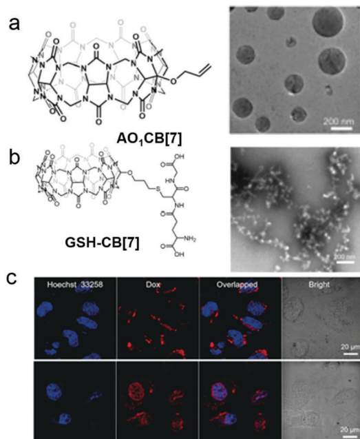
Fig. 17 Chemical structures and TEM images of self-assemblies of (a) AO_1CB[7] and (b) GSH-CB[7] . (c) CLSM images of DOX@AO_1CB[7] vesicle treated HeLa cells without (top) and with (bottom) irradiation by a laser ( \lambda = 720 nm). Adapted with permission from ref. 76. Copyright 2018 John Wiley and Sons.
