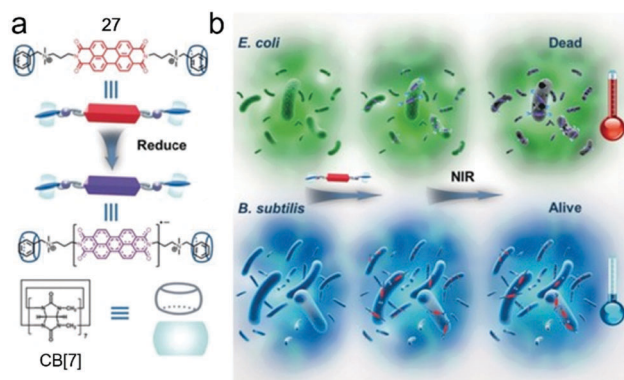
Fig. 19 (a) Chemical structures and formation of the supramolecular radical of CB[7]/27 . (b) Cartoon representation of the selective photothermal therapy for anaerobic bacteria. Adapted with permission from ref. 82. Copyright 2017 John Wiley and Sons.
