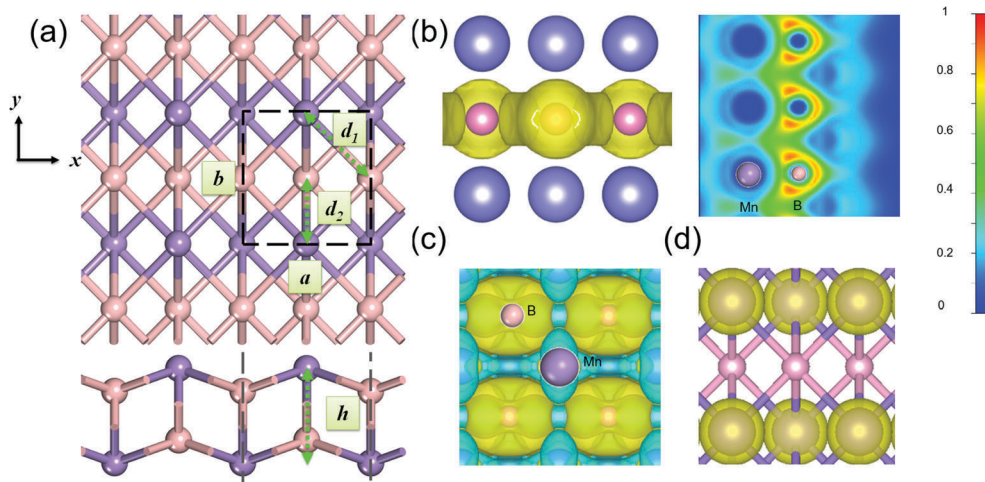
Fig. 1 (a) Top and side views of a 2D MnB sheet; a and b are the lattice parameters, and h denotes the thickness of the layer. (b) Maps of the electron localization function (ELF) located on the (0\ -1\ -6) plane with a scale bar from 0 to 1. (c) The deformation density of the MnB sheet with an isosurface of 0.01\text{ e}\ \text{\AA}^{-3} . The yellow and cyan regions represent the accumulation and depletion of electrons, respectively. (d) The spin polarization distribution with an isosurface of 0.75\text{ e}\ \text{\AA}^{-3} . The yellow color indicates a net spin-up polarization, and the spin polarization is mainly on the Mn sites.
