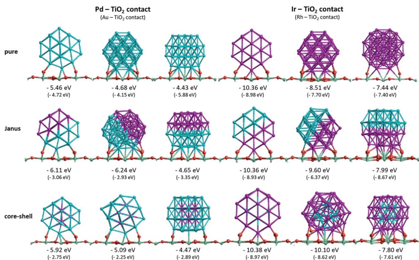
Fig. 5 Structures and corresponding surface binding energies ( E_{s\text{-bind}} ) for 38-TO pure Pd and Ir clusters and Pd–Ir nanoalloys supported on \text{TiO}_2(110) in three orientations. The surface binding energies of Au–Rh clusters, corresponding to the same structures (with Au replacing Pd and Rh replacing Ir), are given in parentheses. Pd, Ir, O and Ti atoms are represented in blue, purple, red and green, respectively. For simplicity, only the top layer of the \text{TiO}_2 slab is shown.
