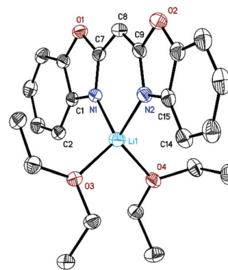
Fig. 1 Molecular structure of [(\text{NCOC}_6\text{H}_4)_2\text{CH})\text{Li}(\text{OEt}_2)_2] ( 1 ). Anisotropic displacement parameters are depicted at the 50% probability level. Hydrogen atoms are omitted for clarity. Structural data are given in Table 1 and the Experimental.
