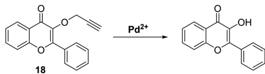
Scheme 19 Propargyl-protected probe 18 for the ratiometric fluorescence detection of Pd 2+ . Measurement conditions: HEPES/ACN (4 : 1).
