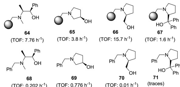
Fig. 10 General structures of supported Ti-TADDOLates and of supported \beta -aminoalcohols and their N -benzylated homogeneous analogues.
