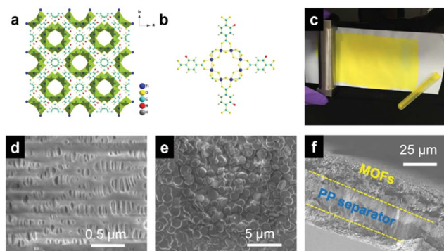
Fig. 1 MOF-decorated separator. (a) Illustration of the structure of NH 2 -MIL-125(Ti). (b) One node of the MOF structure. (c) MOF film coated on PP separator membrane. (d) Top-view SEM image of the pristine separator. (e) Top-view SEM image of the MOF-decorated separator. (f) Cross-sectional view of MOF-decorated separator.
