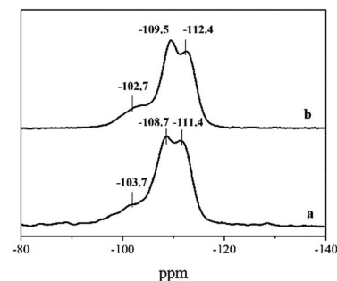
Fig. 5 ^{29}\text{Si} MAS NMR spectrum of (a) 6C-DMP-MTW, (b) 6C-DEP-MTW.
