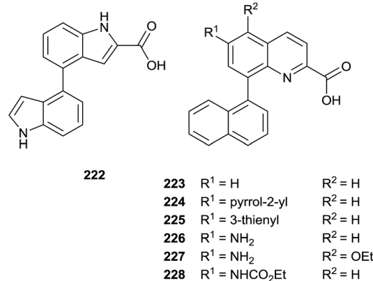
Fig. 6 Quinoline substrates.
