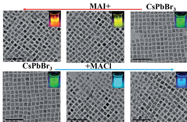
Fig. 4 TEM images of the CsPbBr 3 NCs after treatment with various quantities of MAI (up) and MACl (down). The insets show the evolution of emission colors (under a UV lamp, \lambda_{\text{ex}} = 365 nm) from crude CsPbBr 3 NCs to composited perovskite NCs. Scale bars correspond to 50 nm.
