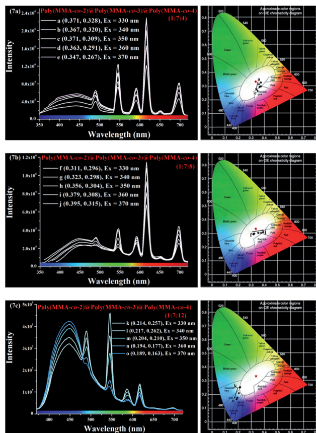
Fig. 7 Emission spectra (left) and corresponding CIE coordinates (right) of polymers' blends Poly(MMA-co-2)@Poly(MMA-co-3)@Poly(MMA-co-4) with different doping mass ratios (1 : 7 : 4, 1 : 7 : 8 and 1 : 7 : 12) in the solid state at room temperature upon excitation: (7a) 1 : 7 : 4; (7b) 1 : 7 : 8; (7c) 1 : 7 : 12.
