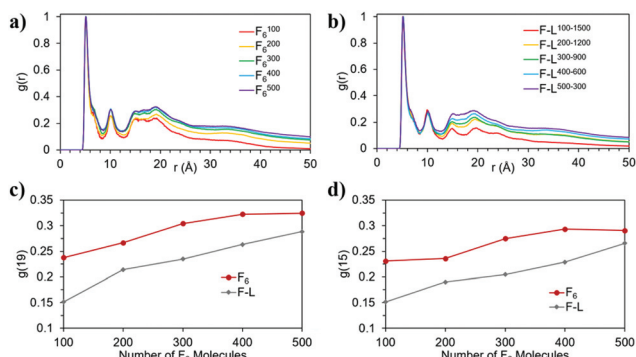
Fig. 4 Normalized RDF of the F_6 molecules in the (a) control and (b) co-assembly simulation; and evolution of the RDF analysis, g(r) , at (c) r = 19 and (d) r = 15 for the control ( F_6 ) and co-assembly ( F-L ) systems as a function of the number of F_6 molecules.
