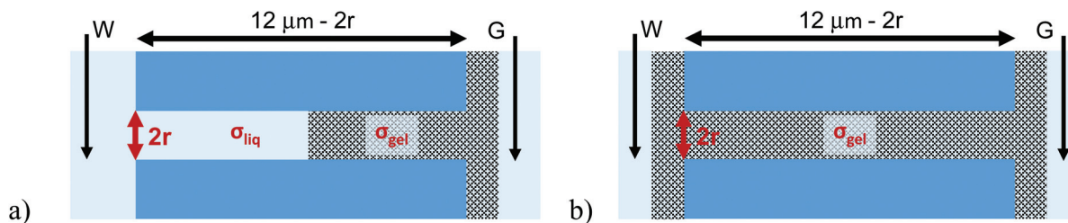
Fig. 1 Scheme of experiments in which single pore membranes subjected to (a) one-sided or (b) double-sided gel dropping were placed in contact with liquid electrolyte of LiClO 4 in propylene carbonate. Note the regions containing the working and counter electrodes are macroscopic reservoirs with liquid electrolyte thus they do not significantly contribute to the system resistance. W and G indicate working and ground electrodes, respectively. The penetration length in (a) is not known, here schematically it is marked as approximately half of the pore length.
