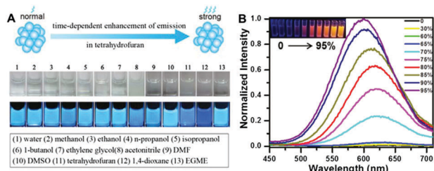
Fig. 5 (A) Solvent effect on PEI protected Cu NCs; (B) PL emission spectra (excited at 365 nm) of Cu NCs in the mixture of water and ethanol with different percentages of ethanol (noted on the frame); inset picture presents a photograph of the respective solution under UV light, demonstrating their increasing emission intensity due to the AIE effect. (A) Reproduced with permission from ref. 105, Copyright 2015, American Chemical Society.
