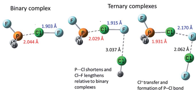
Fig. 4 Computational models of complexes \text{H}_2\text{FP}\cdots\text{ClF} , \text{H}_2\text{FP}\cdots\text{ClF}\cdots\text{HCl} and \text{H}_2\text{FP}\cdots\text{ClF}\cdots\text{ClF} , illustrating co-operativity in halogen bonding interactions. Adapted from DOI: 10.1039/c7fd00048k with permission from The Royal Society of Chemistry.
