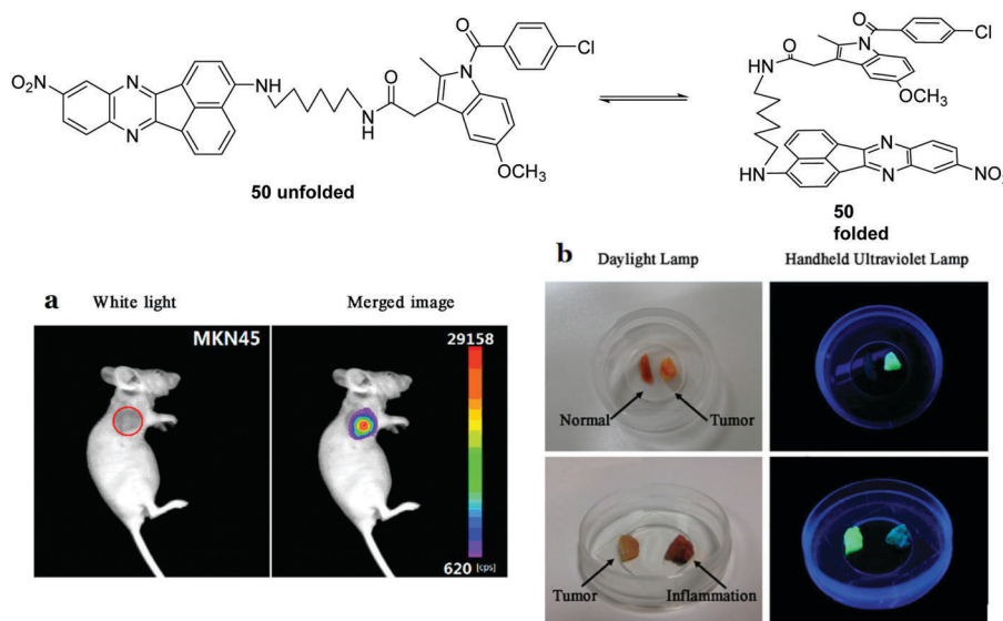
Fig. 29 Structures of the fluorescent chemosensors 50 and imaging tumors in vivo . (a) 50 (30 \mu M) was injected intravenously (30 \mu L). The incubation time was 30 min. (b) Visualization of tumor resection by the naked eye under ultraviolet illumination. Reproduced from ref. 47 with the permission of the American Chemical Society.
