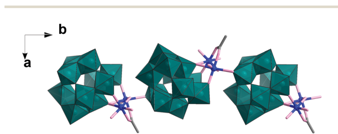
Fig. 2 Representation of the polyanion chain structure of 2 . The \{W_{11}\} building units are shown as teal polyhedra, Cu as blue ball, O and C as rose and grey sticks.
