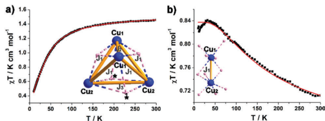
Fig. 4 Temperature dependence of \chi_M T for 1 (a) and 2 (b) from 2–300 K at 500 Oe. Solid lines represent best fits to a Heisenberg-only model. Inset: Exchange connectivity within the cubic \{Cu^{II}_4\} unit in 1 and dimer \{Cu^{II}_2\} unit in 2 ( Cu^{II} blue spheres, all other corners/intersections represent \mu -oxo groups, * represents the oxygen from acetate) illustrating the six principal superexchange pathways in 1 and one principal superexchange pathways in 2 : J ( Cu^{II} – Cu^{II} , light orange lines).
