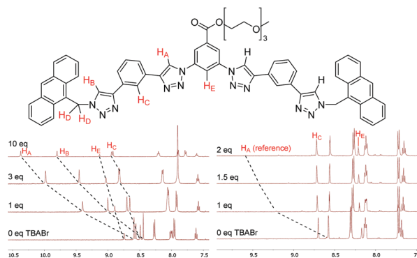
Fig. 2 Top: Labeling of protons monitored in ^1H NMR anion binding studies (consistent across 1–4 ). Bottom left: Partial ^1H NMR spectra of 2a titrated with TBABr. Bottom right: Partial ^1H NMR spectra of a competition experiment where 2b with 5 mol% of 2a as reference is titrated with TBABr (500 MHz, CDCl_3 , 298 K).
