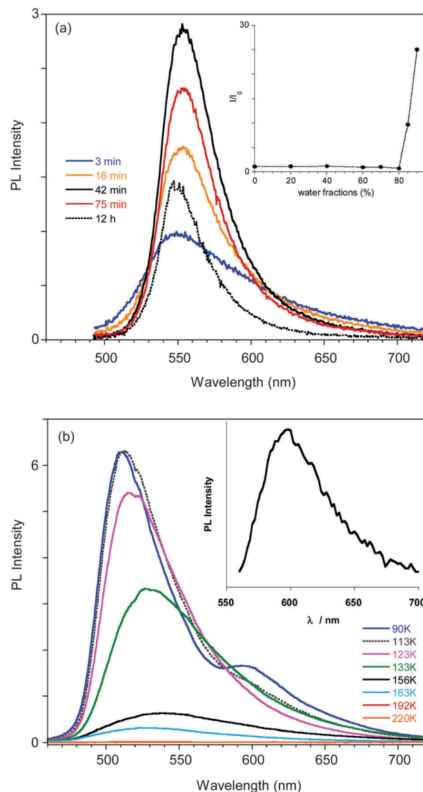
Fig. 2 (a) Emission spectra of a solution of 1 in acetone/ \text{H}_2\text{O} (concentration 1 \times 10^{-5} M) with 85% water measured at different delay times from water addition. In the inset the intensity of the emission for different water fractions (normalized with respect to the intensity at 0% water) is reported, as measured just after water addition. (b) Emission spectra of a THF solution of 1 at different temperatures. In the inset the PL emission at 77 K measured at 2.5 \mu\text{s} delay is reported.
