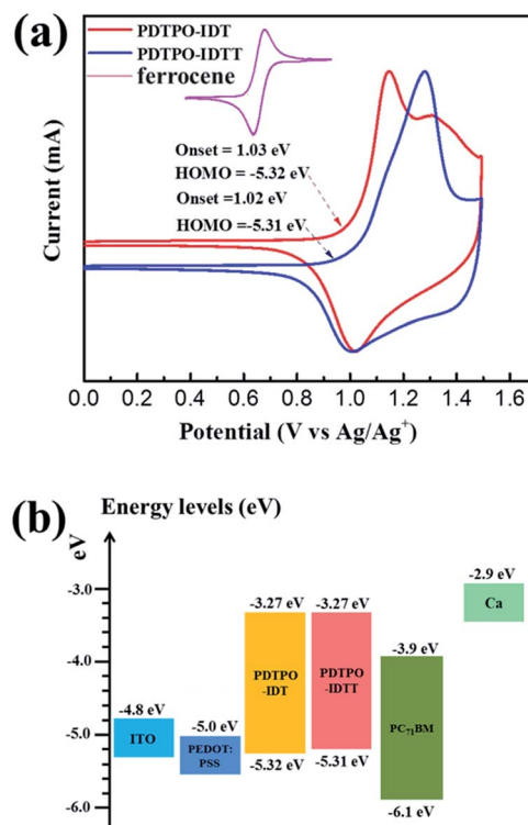
Fig. 2 (a) The electrochemical cyclic voltammetry measurements of PDTP0-IDT and PDTP0-IDTT thin film coated on the platinum electrode in acetonitrile solution containing 0.1 M n\text{-Bu}_4\text{NPF}_6 at a scan rate of 100 \text{ mV s}^{-1} . (b) Schematic energy level diagram of all components used in conventional devices.
