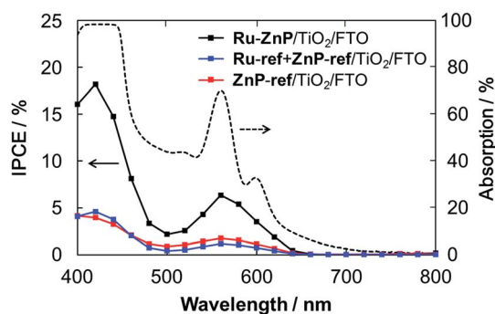
Fig. 5 Photocurrent action spectra of the Ru-ZnP/TiO 2 /FTO (black), Ru-ref + ZnP-ref/TiO 2 /FTO (blue) and ZnP-ref/TiO 2 /FTO electrodes with a TiO 2 thickness of 6 \mu\text{m} . Dashed line depicts the light-harvesting efficiency of the Ru-ZnP/TiO 2 /FTO electrode. Conditions: external bias: -0.2 \text{ V} vs. NHE, electrolyte: PB (0.1 M, initial pH 7.3); and scan rate: 2 \text{ nm s}^{-1} from 400 nm to 800 nm.
