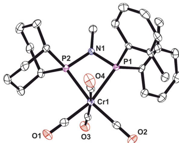
Fig. 9 Crystal structure of [Cr(CO)_4(L_g)] ( 8 ). All hydrogen atoms have been omitted for clarity. Selected bond lengths (Å) and angles (°): Cr(1)–P(1) 2.3477(6), Cr(1)–P(2) 2.3669(6), P(1)–N(1) 1.7146(17), P(2)–N(1) 1.7035(17), P(1)–Cr(1)–P(2) 68.04(4), P(2)–N(1)–P(1) 101.01(9), N(1)–P(1)–Cr(1) 94.67(6), N(1)–P(2)–Cr(1) 94.29(6), C(16)–P(1)–C(13) 95.66(10), C(7)–P(2)–C(4) 105.17(9).
