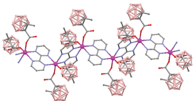
Fig. 22 Infinite polymer chain of the hybrid [\text{Mn}(1\text{-CH}_3\text{-}2\text{-CO}_2\text{-}1,2\text{-closo-C}_2\text{B}_{10}\text{H}_{10})_2(\text{bpm})]_n (81) (H atoms omitted by clarity).
