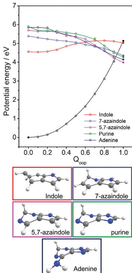
Fig. 13 Overlaid diabatic PECs along Q_{oop} for the {}^1\pi\pi^*/S_0 state that correlates with the {}^1\pi\pi^*/S_0 MECI in indole, 7-azaindole, 5,7-azaindole, purine and A. The filled points show the energies of the optimised critical structures (i.e. the S_0 state minimum and the S_0/{}^1\pi\pi^* MECI) and, for clarity, only the S_0 PEC calculated for indole is shown (open black points). The optimised geometry at each MECI is shown below.
