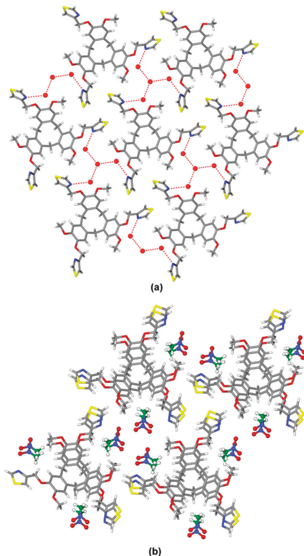
Fig. 1 Clathrate complexes of L . (a) 2D hydrogen bonded network from crystal structure of L ·4( \text{H}_2\text{O} ) viewed down c axis. Water shown as spheres, \text{N}\cdots\text{O} and \text{O}\cdots\text{O} separations are 2.895 and 2.918 Å respectively. (b) Packing diagram of L ·3( \text{CH}_3\text{NO}_2 ) with \text{CH}_3\text{NO}_2 shown in ball-and-stick.
