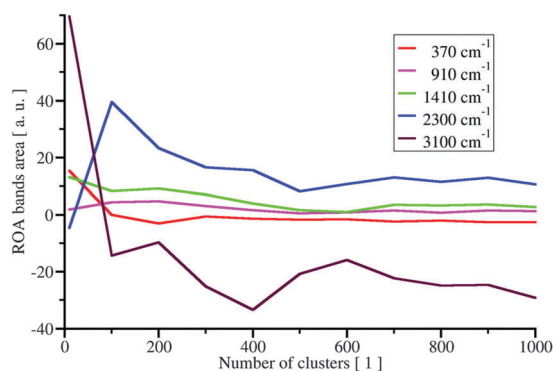
Fig. 5 Intensities of selected simulated ACN ROA peaks dependent on the number of clusters taken into averaging within the TPM approach (peaks at different wavenumbers in cm⁻¹ are indicated by color code). For example, in the case of the CN band at 2300 cm⁻¹ (blue), the intensity remains essentially constant when more than 400 clusters are averaged. In our TPM model, 1000 clusters were used for simulation of spectra.
