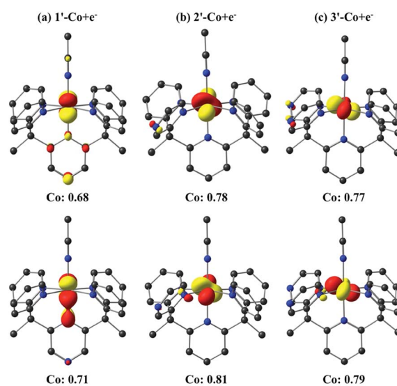
Fig. 9 Isosurface (0.07 au) plots of the canonical highest occupied molecular orbitals (HOMOs, top) and \beta -spin localized orbitals (bottom) for 1'\text{-Co} + \text{e}^- , 2'\text{-Co} + \text{e}^- and 3'\text{-Co} + \text{e}^- ( S = 1 ). The Löwdin population analyses are given for cobalt.
