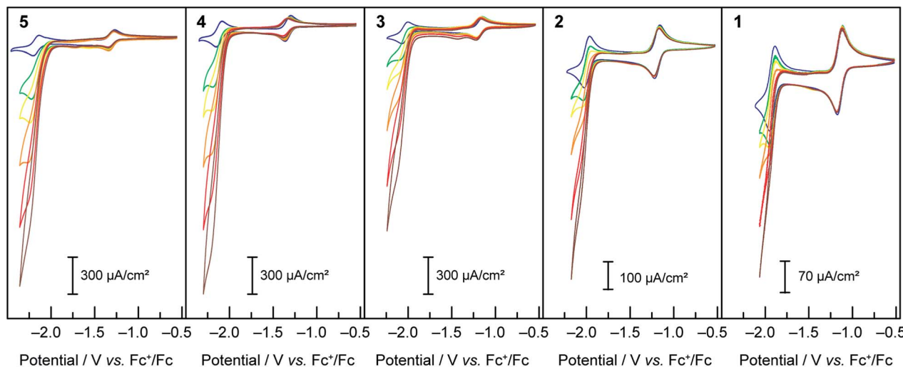
Fig. 2 Cyclic voltammograms under Ar at 50 \text{ mV s}^{-1} of 1 mM solutions of compounds 1–5 in DMF, TBAPF 6 0.1 M, on a glassy carbon electrode with 0 (— blue), 5 (— green), 10 (— yellow), 20 (— orange), 40 (— red) and 60 (— brown) mM of acetic acid.
