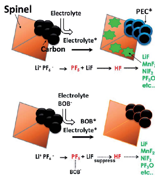
Fig. 15 Proposed mechanism of the LiBOB additive for the improvement in electrochemical performance of the spinel high-voltage LNFMO cathode. Reproduced with permission. 69
