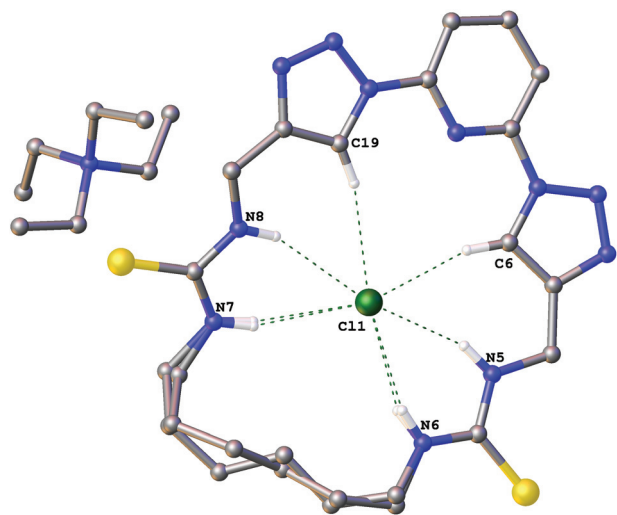
Fig. 1 The crystal structure of 6a \cdot (TEA^+) \cdot (Cl^-) . Non-acidic hydrogen atoms have been omitted for clarity and hydrogen bonds are shown as dashed lines.
