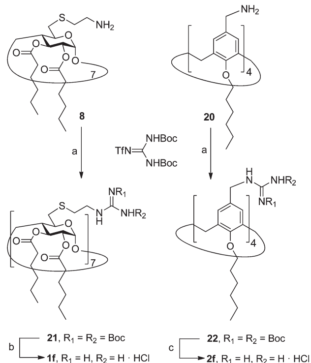
Scheme 4 Synthesis of polyguanidino \beta CD and CA_4 derivatives 1f and 2f . Reagents and conditions: (a) TfN, DCM, rt, 12 h, 99% (for 21 ) or 48 h, 91% (for 22 ); (b) (i) 1 : 1 TFA-DCM, rt, 3 h; (ii) 0.1 M HCl, 99%; (c) TES, dioxane, 0.1 M HCl, rt, 24 h, quantitative.
