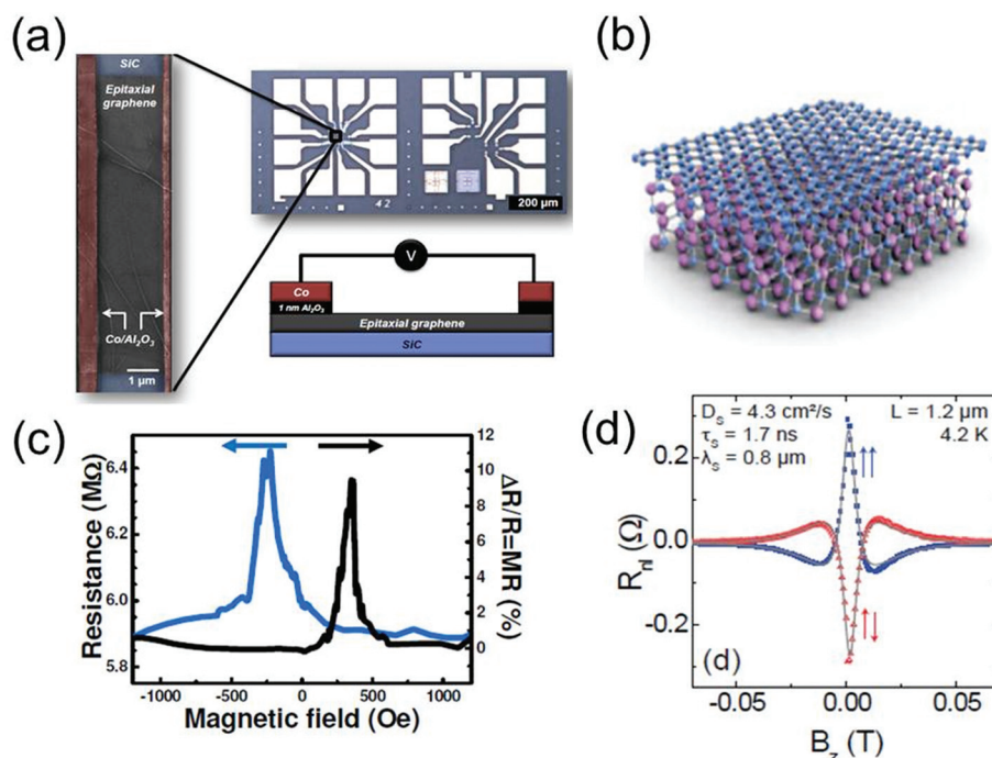
Fig. 71 (a) Typical two-terminal local spin valve device. The width of graphene channel on SiC is 10 μm, and the distance between the two Al 2 O 3 /Co electrodes is L = 2 \mu\text{m} . The optical image shows the entire structure, including contact pads. (b) Atomic arrangement of SLG on SiC. (c) Large local resistance spin signals measured at 4 K. (d) Oscillating and decaying device non-local resistance as a function of the applied magnetic field (Hanle measurement). Adapted from ref. 223, 1300.
