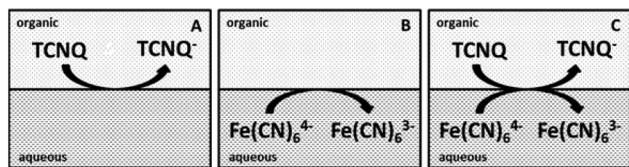
Scheme 2 Diagrams of the cells for the ET studies. (A) The organic blank for cell 3, (B) the aqueous blank for cell 4, (C) both redox species in the aqueous and organic phases for cell 5.
