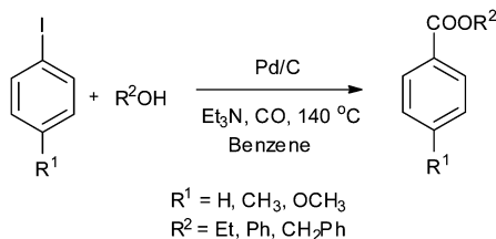
Scheme 37 Reagents and conditions: aryl iodide (2.5 mmol), alcohol (2.5–3.0 mmol), Et 3 N (3 mmol), 5% Pd/C (50 mg), benzene (5 mL), carbon monoxide (1 MPa), temp. 140 °C, time 6 h.
