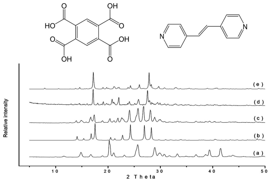
Fig. 15 Demonstration of the enhanced kinetics of cocrystal formation upon addition of a few drops of methanol to the grinding jar. PXRD patterns for (a) tetracarboxylic acid, (b) bipridyl, (c) outcome of neat grinding for 60 minutes (as the sum of the reactants), (d) the product obtained when a few drops of methanol are added and (e) the simulated pattern for the cocrystal.
