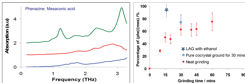
Fig. 2 (a) Terahertz spectra obtained from (top to bottom): a 1 : 1 mesoconic acid–phenazine cocrystal; mesoconic acid; phenazine. (b) Analysis ( ex situ ) of the extent of formation of the cocrystal from a mixture of phenazine and mesoconic acid, as a function of neat grinding time, as measured using the characteristic cocrystal band at 1.1 THz (red circles). The blue star, by comparison, shows close to 100% conversion in 15 minutes as a result of the presence of liquid in a LAG experiment. The blue square represents the percentage of a cocrystal sample that remained crystalline during dry grinding. 56
