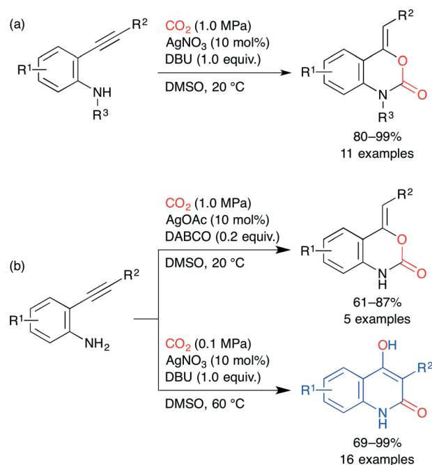
Scheme 20 The Ag-catalyzed incorporation of \text{CO}_2 into o -alkynylanilines.
