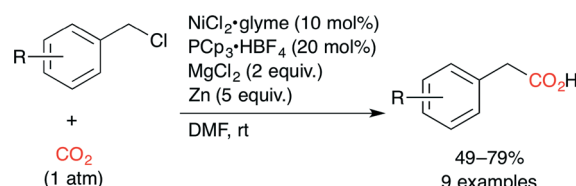
Scheme 8 The Ni-catalyzed carboxylation of benzyl chlorides with CO 2 .
