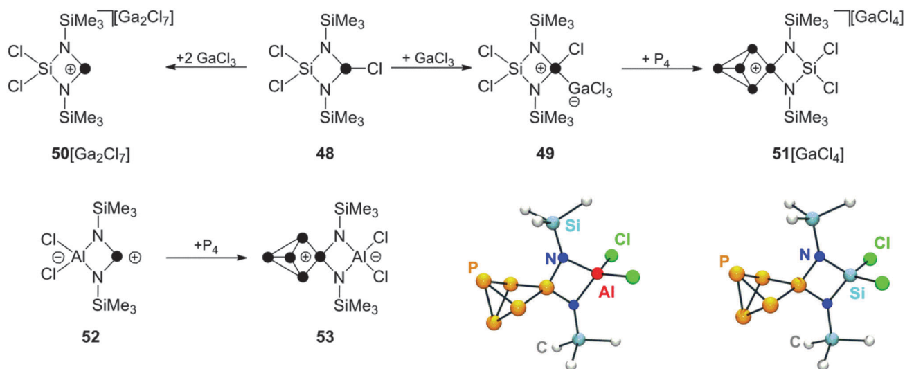
Scheme 14 Preparation of \text{P}_5^+ -cage cation \mathbf{51}^+ from \text{P}_4 , \text{GaCl}_3 and chlorophosphane \mathbf{48} (top) and preparation of zwitterionic \text{P}_5 -cage compound \mathbf{53} from \text{P}_4 and zwitterionic phosphonium ion \mathbf{52} .
