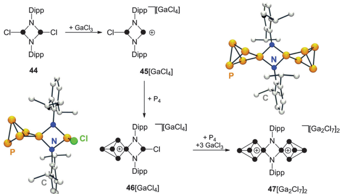
Scheme 13 Stepwise synthesis of \text{N}_2\text{P}_{10} -cage compound \mathbf{47}[\text{Ga}_2\text{Cl}_7]_2 via insertion of phosphonium ions generated in situ by the reaction of diphosphadiazane \mathbf{44} with \text{GaCl}_3 .
