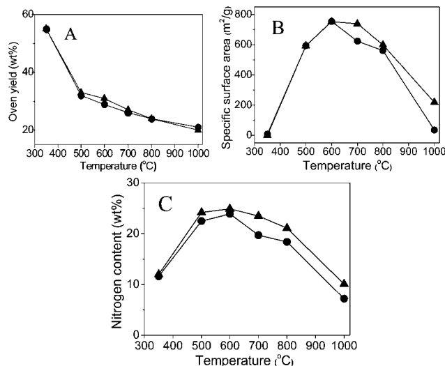
Fig. 1 Plots of carbonization yield (A), specific surface area (B) and nitrogen content (C) vs. carbonization temperature of the carbonized products from the IL monomer \text{CMVImTf}_2\text{N} (solid triangles) and the PIL polymer \text{PCMVImTf}_2\text{N} (solid circles).
