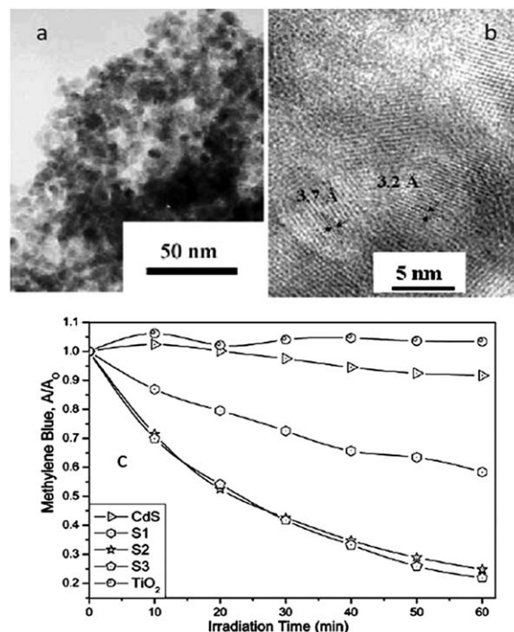
Fig. 10 (a and b) TEM and HRTEM images of CdS/TiO 2 ; (c) the MB degradation under visible light irradiation (660 nm) in the prepared photocatalysts (reprinted with permission from ref. 24, copyright 2003 Royal Society of Chemistry).
