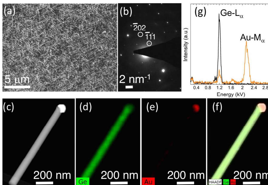
Figure 1. Morphology and composition of the starting Ge nanowires. (a) SEM overview image of the ensemble of Ge nanowires grown by a VLS process in \text{Ge}_2\text{H}_6 over Au catalyst particles on Ge (100) substrates. (b) Electron diffraction pattern of the Ge NW in (b) along the [101] zone axis. (c) High-angle annular dark-field (HAADF) STEM image of a representative Ge NW near the Au-rich tip after transfer onto amorphous carbon film. (d) – (e) EDS chemical maps of the Ge NW showing the distribution of Ge (green) and Au (red). (f) Overlaid Ge and Au maps. (g) EDS spectra obtained along the NW (black) and at the Au-rich NW tip (orange), respectively.
