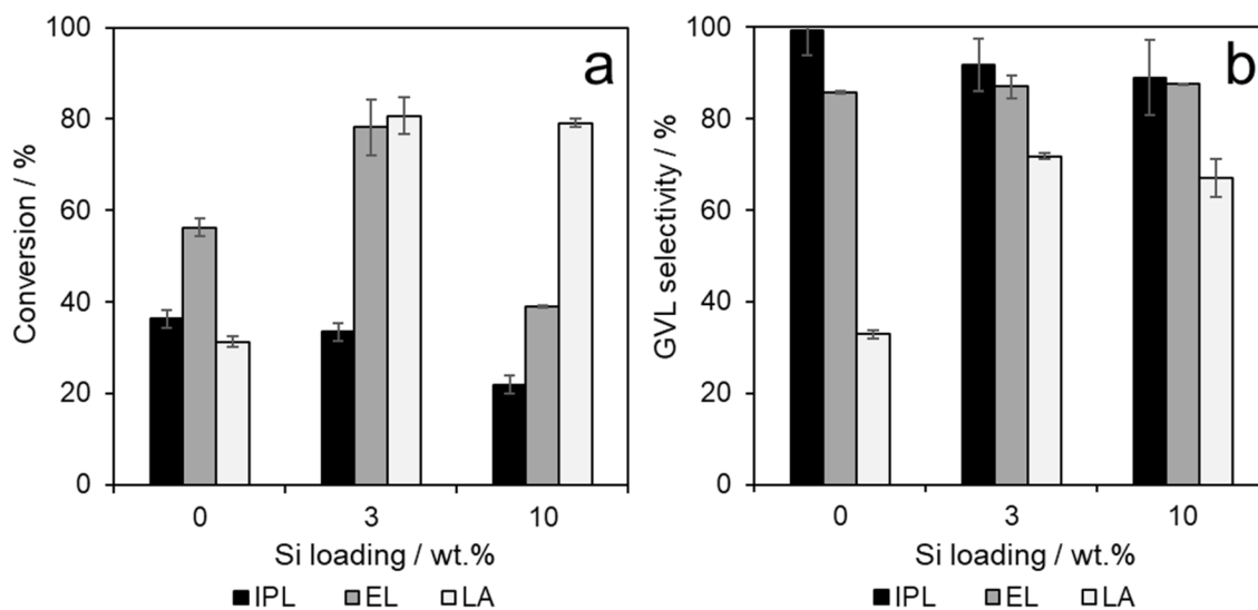
Fig. 10 Reactivity of IPL, EL and LA under CTH conditions. (a) IPL, EL and LA conversion, (b) GVL selectivity from IPL, EL and LA using Si/Zr catalysts. Reaction conditions: catalyst (100 mg), IPL, EL or LA (5 mmol), 2-propanol (250 mmol), internal standard ( n -dodecane, 0.5 mmol), 5 bar N 2 , 170 °C, 6 h.
