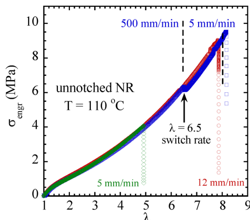
Fig. 10 Stress vs. stretch ratio curves of three NR unnotched dogbone-shaped specimens. Two of the samples were under continuous stretch at constant speed of 5 mm min -1 and 12 mm min -1 , respectively. The other was stretched at 500 mm min -1 till \lambda = 6.5 when NR was further stretched at a slower speed of 5 mm min -1 .
