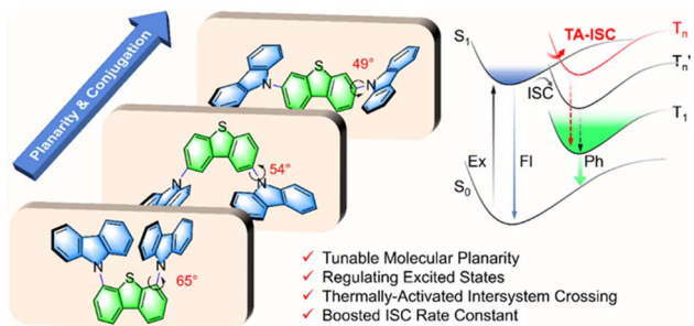
Scheme 1 Diagram of molecular structural engineering and the impact of enhanced-planarity and conjugation on intersystem crossing for achieving efficient organic RTP within a donor–acceptor–donor ternary \pi -conjugated framework.
