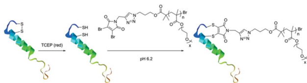
Fig. 14 sCT disulfide bridging with ATRP generated pPGEA via di-bromomaleimide linker. Reprinted with permission from (ref. 125). Copyright 2012 American Chemical Society.
