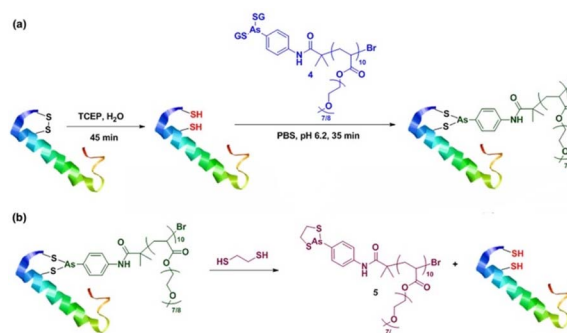
Fig. 15 (a) sCT conjugation to pPGEA via arylarsenous linker. (b) sCT releases in the presence of chelating agent such as EDT. Reprinted with permission from (ref. 135). Copyright 2015 American Chemical Society.
