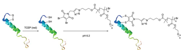
Fig. 14 sCT disulfide bridging with ATRP generated pPGEA via dibromomaleimide linker. Reprinted with permission from (ref. 125). Copyright 2012 American Chemical Society.
