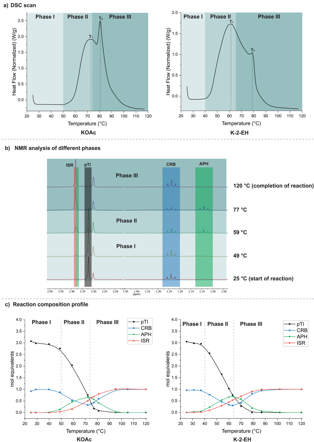
Fig. 2 (a) DSC scans of the model reaction catalyzed by KOAc and K-2-EH, highlighting the distinct phases of the reaction. (b) Representative ^1\text{H} NMR spectra in the chemical shift region of 1.0 to 2.5 ppm, highlighting compositional changes across the phases; spectra shown for KOAc. K-2-EH exhibits a similar trend. (c) Reaction composition profile depicting the phases of the model reaction catalyzed by KOAc and K-2-EH. Reaction: pTI (4.0 equiv.), EE (1.0 equiv.), catalyst (0.375 mol% relative to NCO). DSC conditions: temperature range set as 25 to 120 °C, heating ramp set at 10 °C \text{min}^{-1} . The error associated with sampling at the DSC temperature is estimated to be \pm 2.5 °C.
