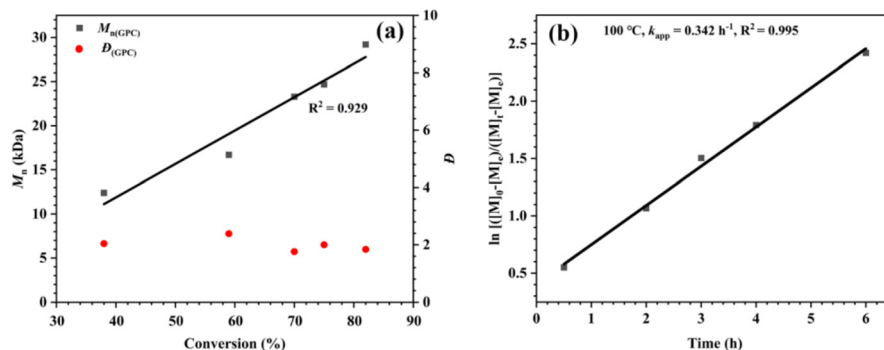
Fig. 1 (a) M n and D of the resultant PDDL versus monomer conversion ([M] 0 /[I] 0 /[C] 0 = 100/1/1, [M] 0 = bulk, T = 100 °C). (b) Kinetic plots of ln{([M] 0 – [M] t )/([M] t – [M] e )} vs. time ([M] 0 /[I] 0 /[C] 0 = 100/1/1, [M] 0 = bulk, T = 100 °C) of DDL.
