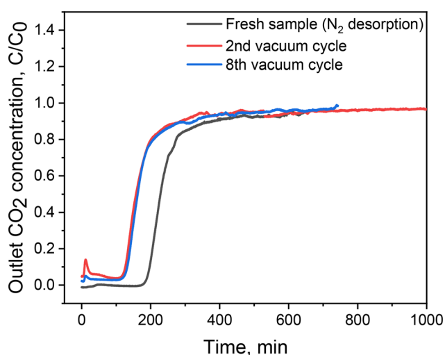
Fig. 10 Breakthrough profiles for TEPA(50)-Mg 2 (dobpdc) under 70% RH and 400 pm CO 2 /N 2 flow (co-adsorption) after vacuum desorption cycles. The adsorption and vacuum desorption experiment cycles consisted of exposing samples to ambient air (22 °C and 50% RH) for 20 h and desorbing adsorbates at 80 °C for 4 h under 0.1 bar static vacuum, followed by transferring the samples after certain cycles (2nd and 8th) to the fixed bed without further desorption. The flow rate was 44 sccm (400 ppm CO 2 /N 2 ).
