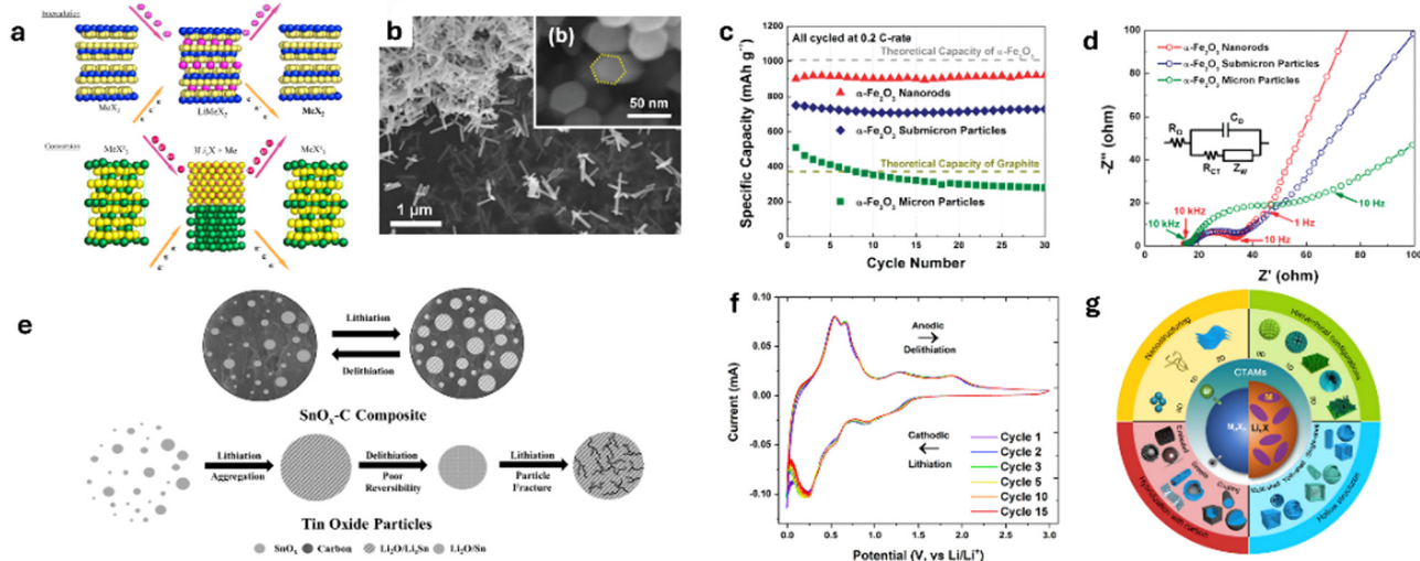
Fig. 21 (a) Comparison of an intercalation and conversion mechanisms for the lithiation/delithiation of electrode materials. Reproduced with permission from ref. 331. Copyright 2007, Elsevier B.V. Illustration of conversion-type electrode lithiation behavior. (b) SEM images of \alpha\text{-Fe}_2\text{O}_3 nanorods at a low magnification and (b) end-view at a high magnification. The yellow dashed line in panel b outlines the hexagonal structure of a single nanorod, (c) reversible capacities of \alpha\text{-Fe}_2\text{O}_3 electrodes made with nanorods, submicrometer particles, and micrometer-sized particles. All electrodes cycled at 0.2C rate (201 \text{mA g}^{-1} ), and (d) electrochemical impedance spectroscopy of electrodes with \alpha\text{-Fe}_2\text{O}_3 nanorods, submicrometer particles \alpha\text{-Fe}_2\text{O}_3 , and micrometer-sized particles \alpha\text{-Fe}_2\text{O}_3 . All measured after 100 cycles at 0.5C rate. Reproduced with permission from ref. 332. Copyright 2011, American Chemical Society. (e) Comparison of \text{SnO}_x\text{-C} lithiation/delithiation versus unsupported tin oxide particle lithiation/delithiation and (f) long-term cyclic voltammograms of \text{SnO}_x\text{-C} . Reproduced with permission from ref. 333. Copyright 2019, American Chemical Society. (g) Schematic Illustration of the nanoengineering strategies for high-performance conversion type anode materials for next-generation LIBs. Reproduced with permission from ref. 25. Copyright 2018, Elsevier Inc.
