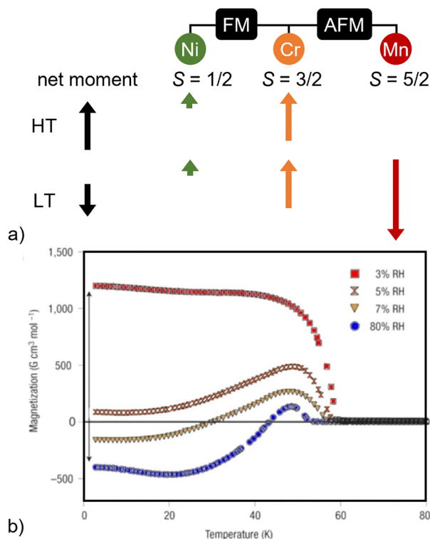
Fig. 5 (a) The evolution of negative magnetisation in \text{Ni}_x\text{Mn}_{1-x}[\text{Cr(CN)}_6]_{2/3} . The magnetic moments of the different ions at high and low temperature (HT/LT) are illustrated. (b) The humidity-sensitive negative magnetisation of \text{Co}_{0.41}\text{Mn}_{0.59}[\text{Cr(CN)}_6]_{2/3} . 82 Reproduced from ref. 82 with permission from Springer Nature.
