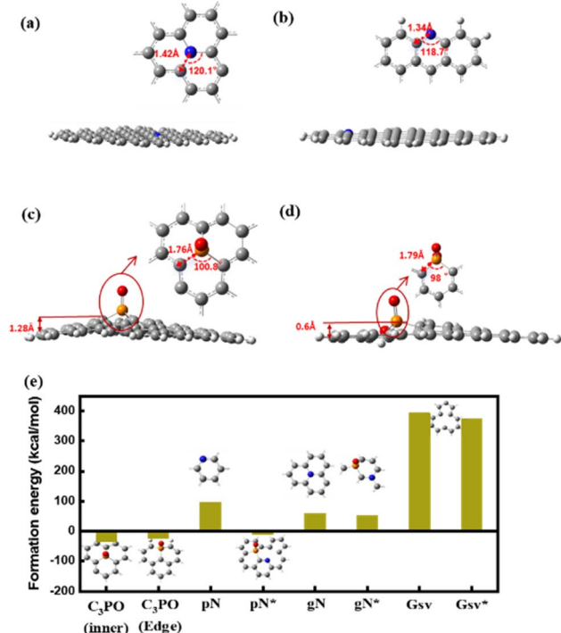
Fig. 6 (a) Optimized models for graphitic N doped graphene. (b) Optimized models for pyridinic N doped graphene. (c) Optimized models for \text{C}_3\text{PO} doped graphene. (d) Optimized models for \text{C}_2\text{PO}_2 doped graphene. (e) The formation energy of the various structures. * represents the generation energy of the structure in the presence of \text{C}_3\text{PO} .
